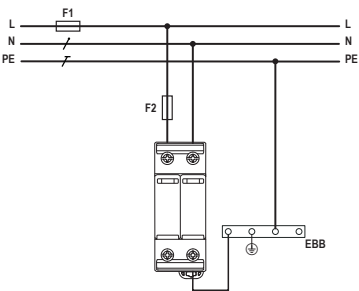
TN-C-S, TN-S Network System, 1+1
