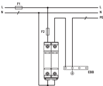
TT Network System, 1+1
